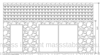
FACHADA PRINCIPAL
