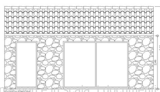
FACHADA PRINCIPAL
