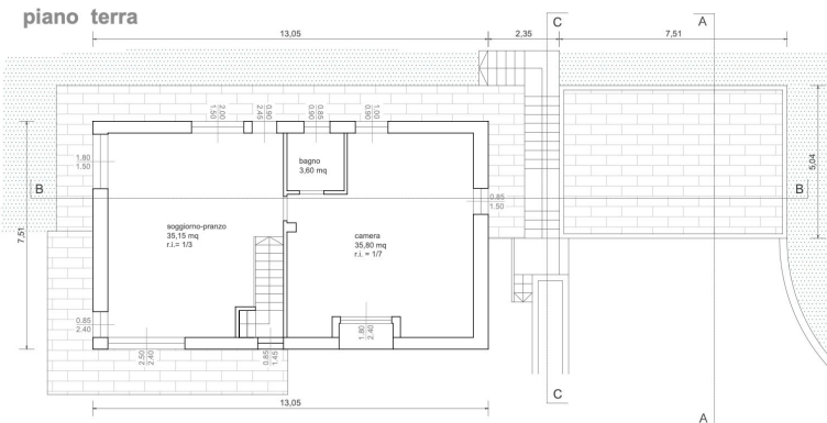
piano terra
