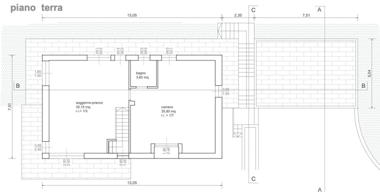
piano terra
